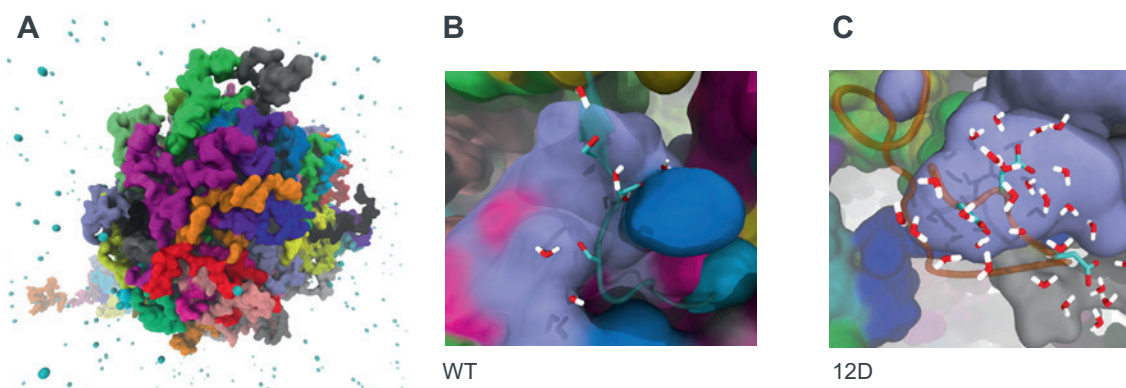
Figure 1. Figure 1. Multi-scale simulations of TDP-43. A) Phase-separated TDP-43 condensate. B) In WT TDP-43, serine residues at the site of the phosphomimicking mutations Ser->Asp interact with other protein residues and with water. C) Aspartate residues at sites of the phosphomimicking mutations Ser->Asp lose many protein-protein interactions, gain only a few charge-charge interactions and interact primarily with water.
