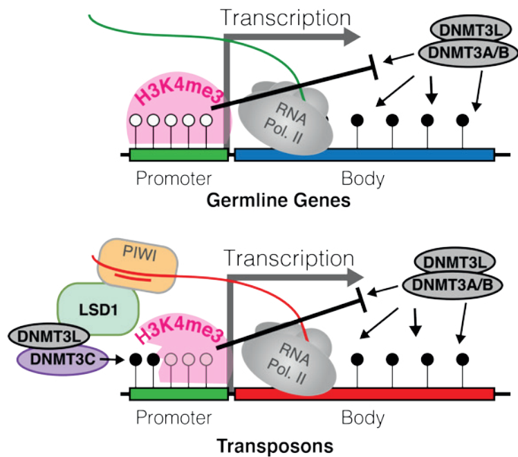
Figure 1. A model for piRNA-guided DNA methylation. De novo methylation of active promoters is prevented due to the repelling effect H3K4me3 has on DNA methyltransferases. TE promoters are recognised by MIWI2, which is loaded with a piRNA, presumably via complementarity of the piRNA to their nascent transcripts. A set of proteins are key to stabilising MIWI2 and initiating silencing (e.g. SPOCD1), however, DNMT3C's interactor LSD1 is responsible for removing inhibitory H3K4me3 and allowing the de novo methylation that ensures stable epigenetic silencing.
