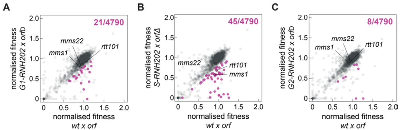
Figure 1. Using synthetic genetic arrays, we screened for mutants that had compromised viability when rNMPs were nicked in either G1 (A), S (B) or G2 (C) phase by expressing cell cycle restricted alleles of RNase H2. Along with Rtt101 and its interacting factor Mms1, many factors involved in HDR and histone deposition were identified as being required to deal with S phase nicks at rNMPs (analysis performed in collaboration with Anton Khmelinskii, IMB).
